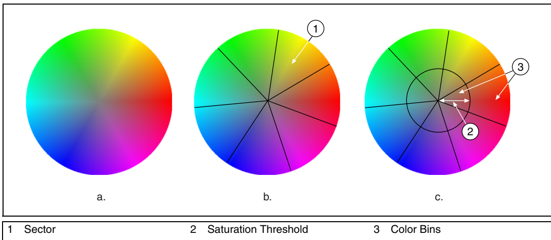
Figure 14-5. The HSL Space Divided into Bins and Sectors
