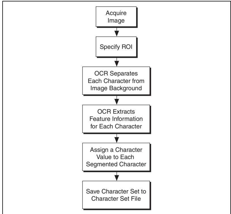
Figure 16-1. Steps of an OCR Training Procedure
