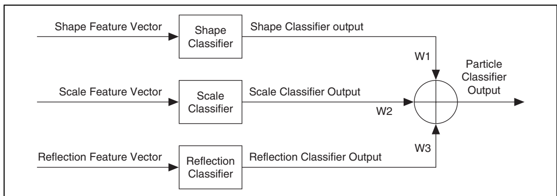
Figure 15-10. Weighted Parallel Classification System
