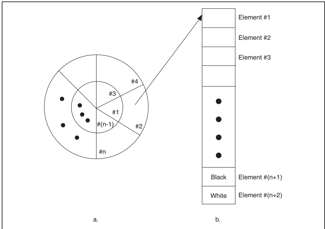
Figure 14-6. Hue Color Space and the Color Spectrum Array Relationship
