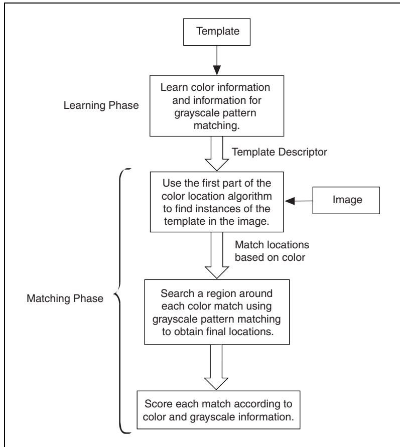
Figure 14-19. Overview of the Color Pattern Matching Process
