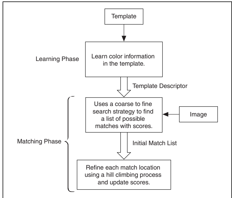
Figure 14-14. Overview of the Color Location Process
