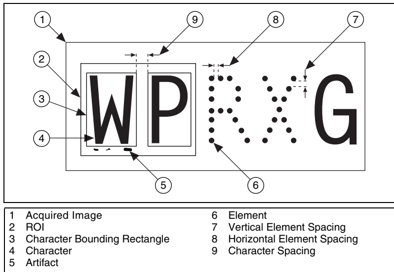
Figure 16-3. Concepts Involved in Character Segmentation
