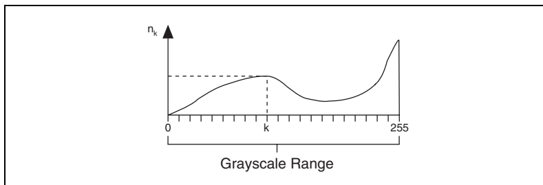
Figure 4-1. Histogram Plot
