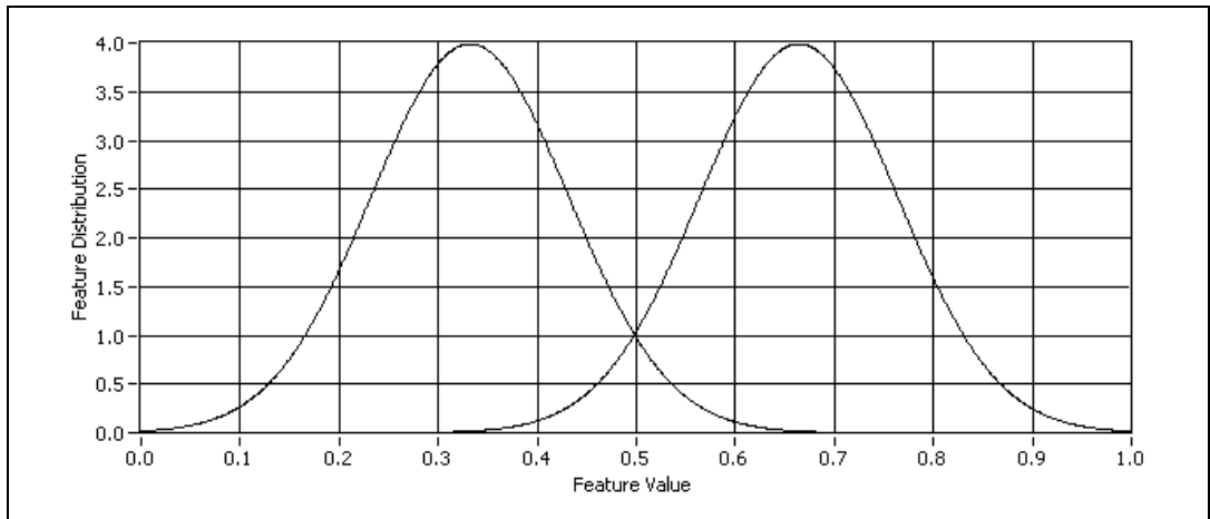
Figure 15-11. Two Classes with Gaussian Distribution
