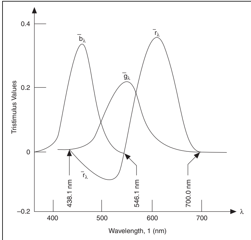
Figure 14-2. Visible Light
