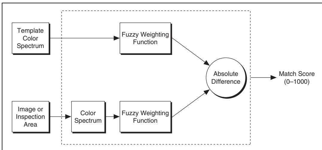
Figure 14-10. Comparing Two Spectrums for Similarity
