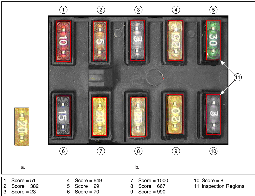
Figure 14-9. Fuse Box Inspection Using Color Matching
