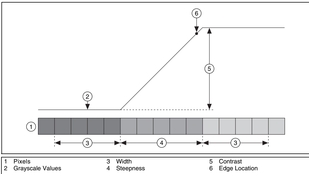
Figure 11-9. Advanced Edge Detection
