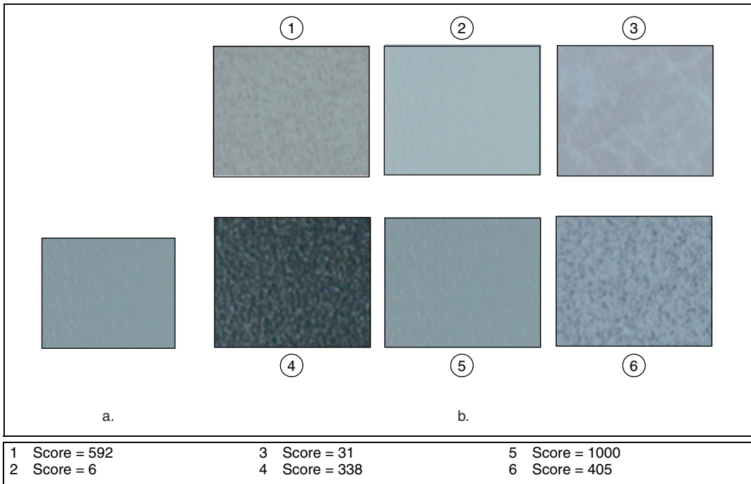
Figure 14-8. Color Matching
