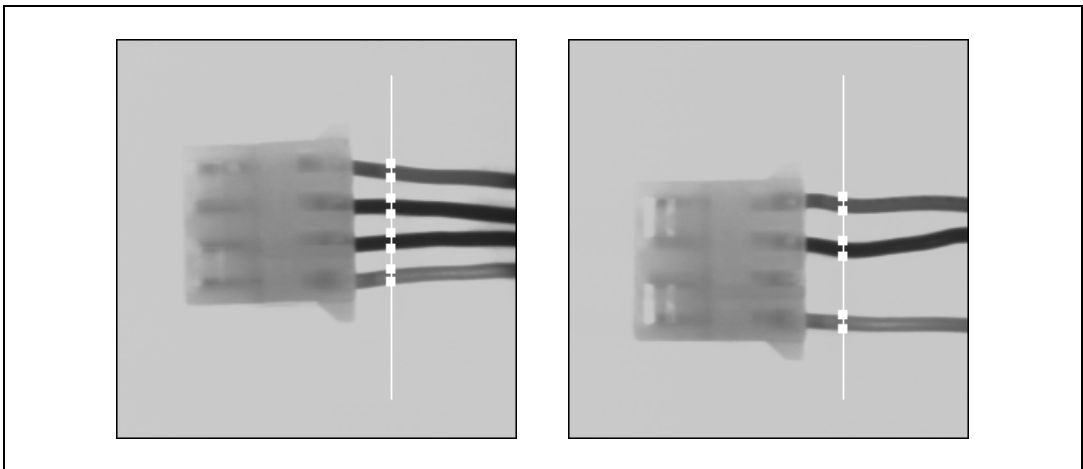
Figure 11-2. Connector Inspection Using Edge Detection
