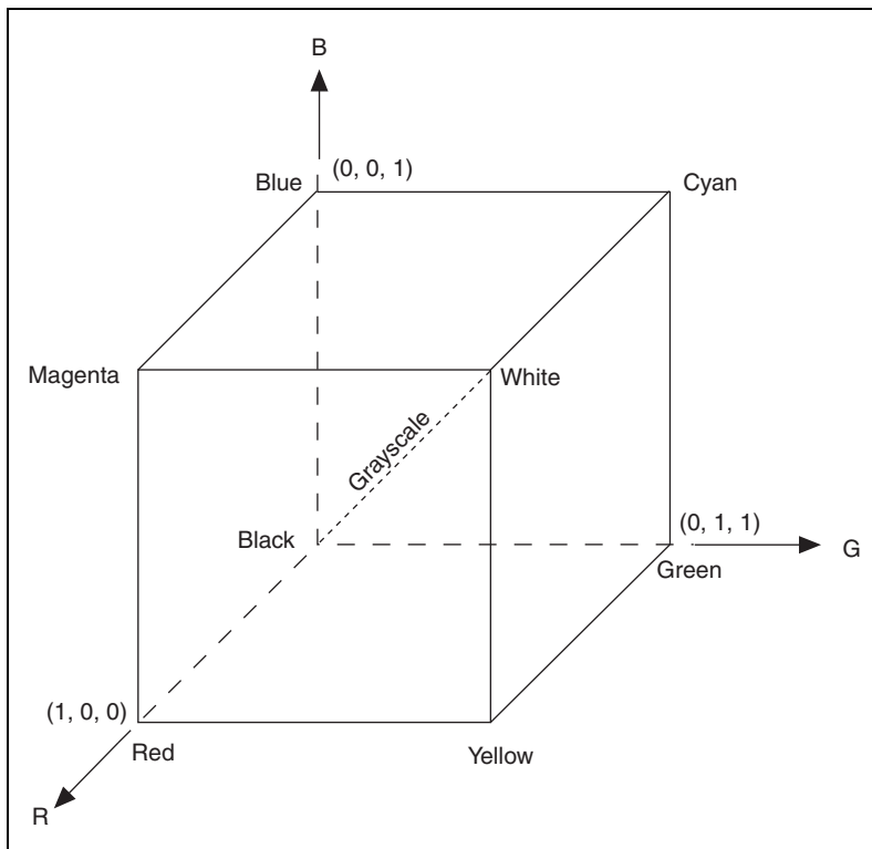
Figure 14-1. RGB Cube
