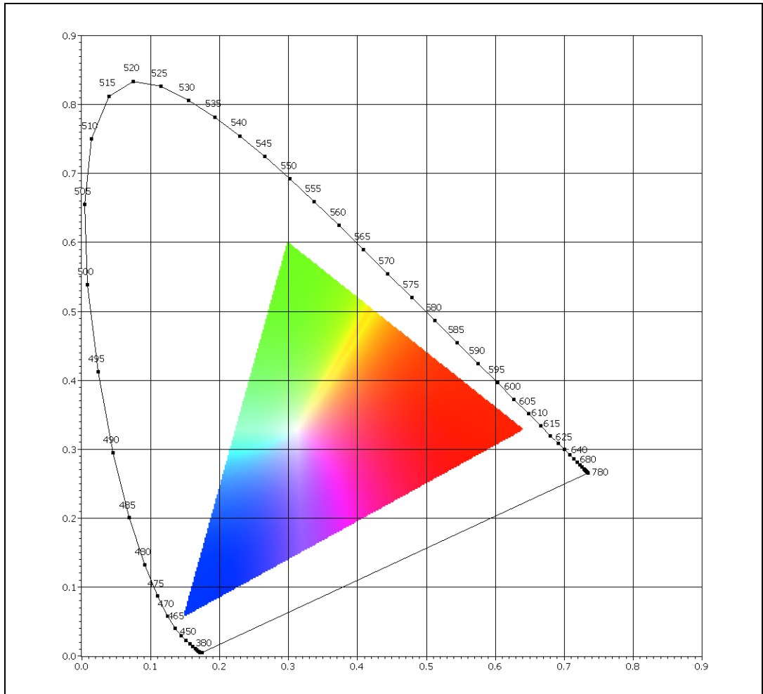
Figure 14-20. CIE Chromaticity Diagram
