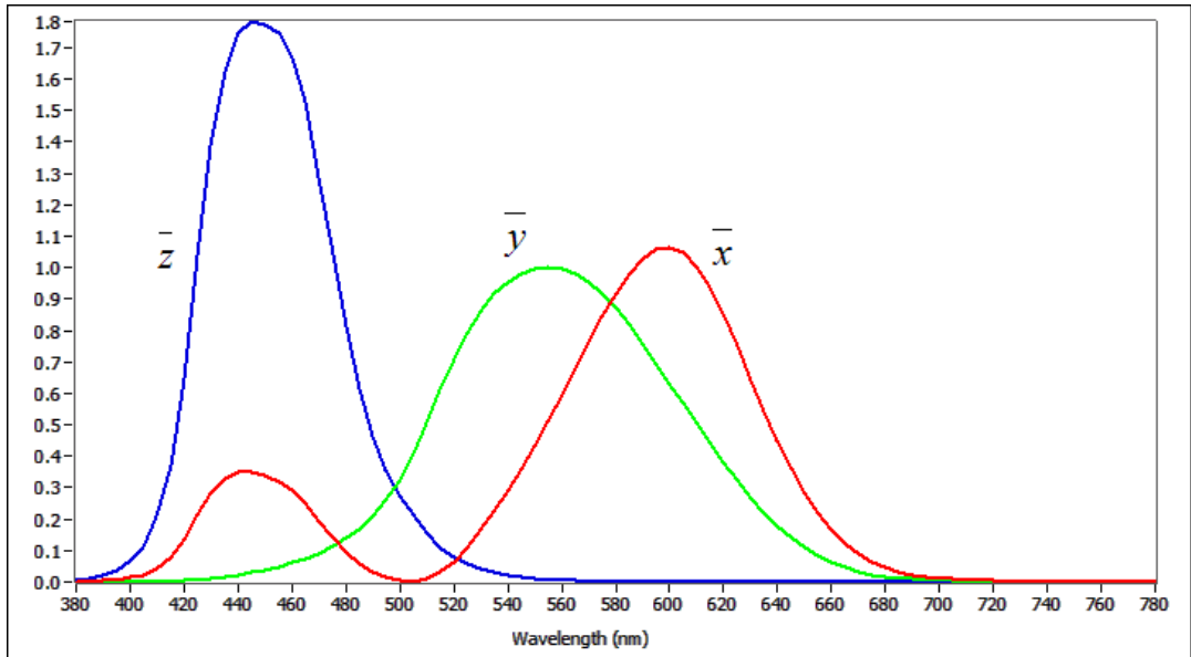
Figure 14-3. CIE Color-Matching Function
