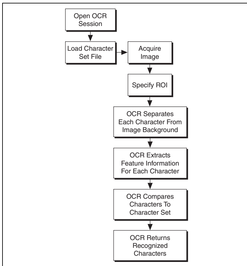
Figure 16-2. Steps of an OCR Reading Procedure
