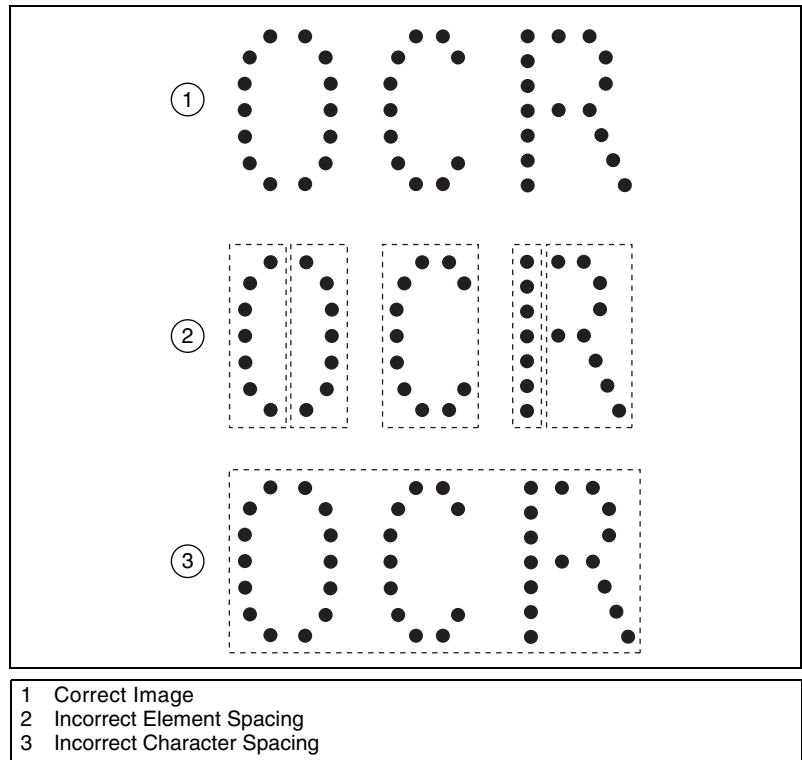
Figure 16-4. Concepts Involved in Character Segmentation
