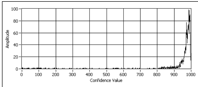
Figure 15-12. Classification Confidence from a Mechanical Parts Database
