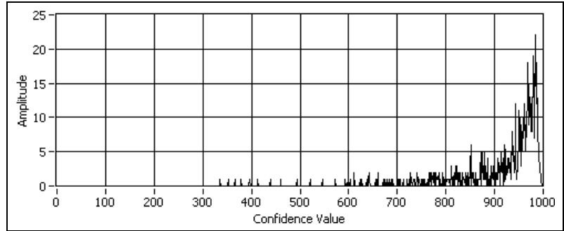
Figure 15-13. Classification Confidence from a Cracker Database
